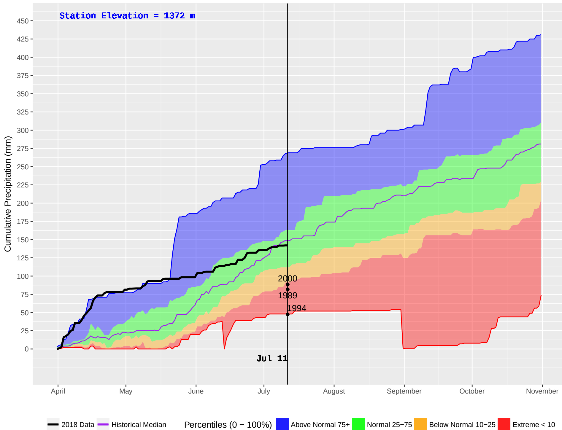
CHERRY LAKE (791) : Historical (1989–2016) and Current (2018) Noon Cumulative Precipitation
