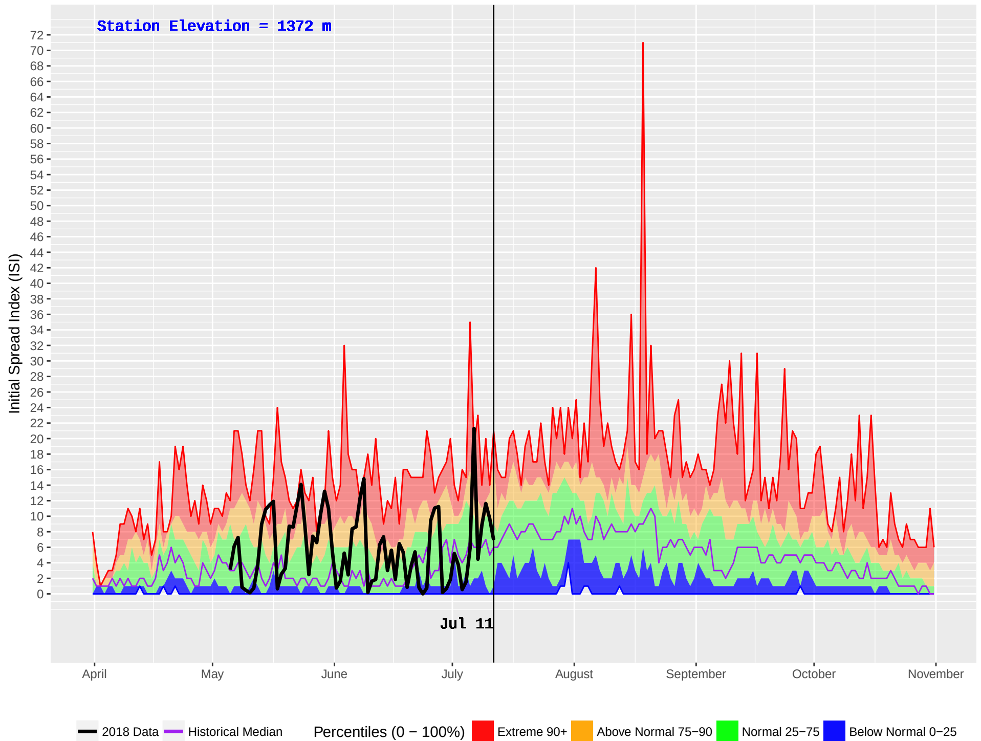
CHERRY LAKE (791) : Historical (1989–2016) and Current (2018) Noon Initial Spread Index (ISI)
