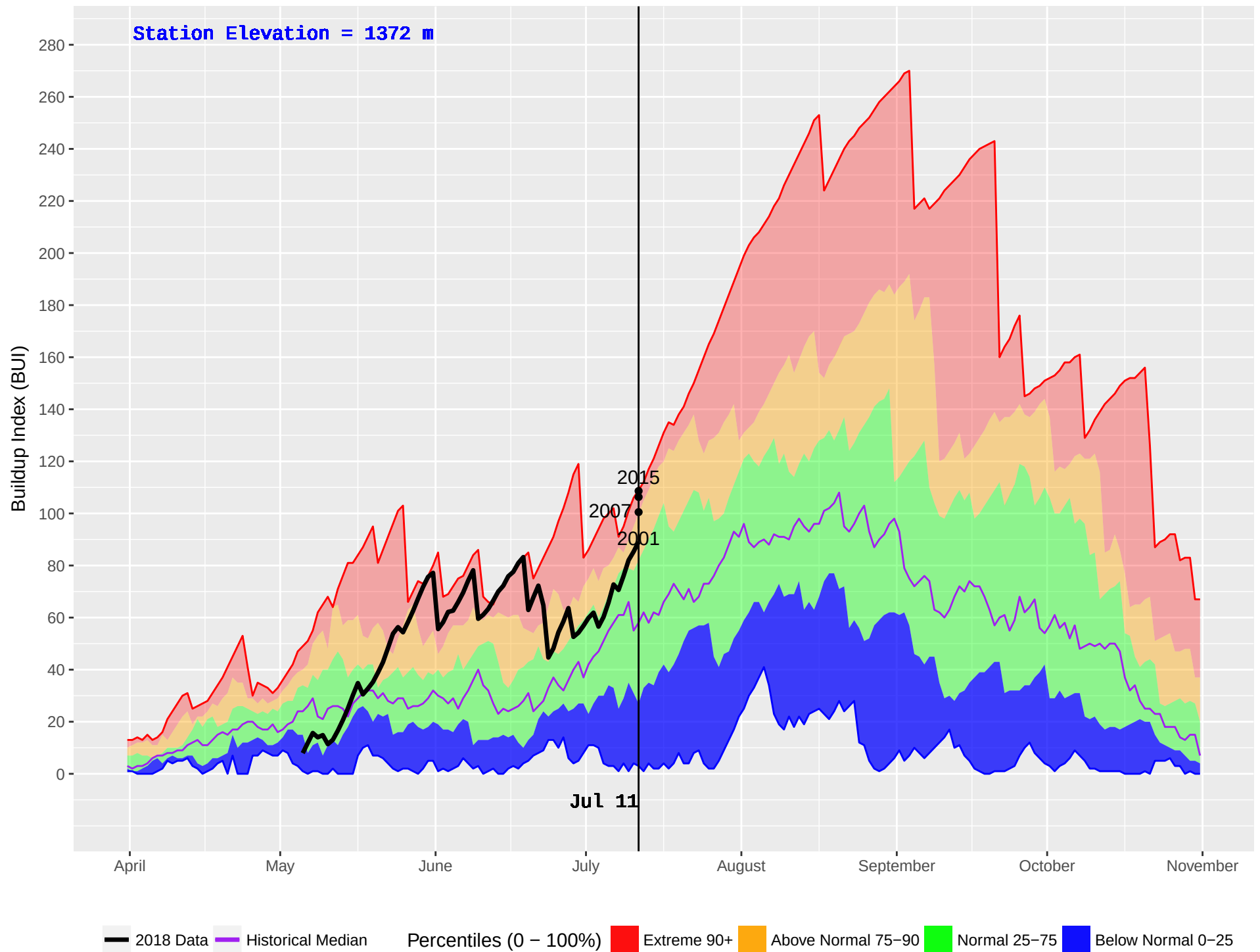
CHERRY LAKE (791) : Historical (1989–2016) and Current (2018) Noon Buildup Index (BUI)
